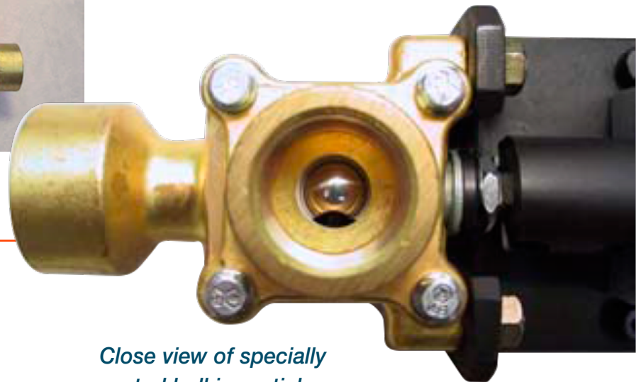
Size 3/4 inch Saint Clair Systems Six way Temperature Control Valve
